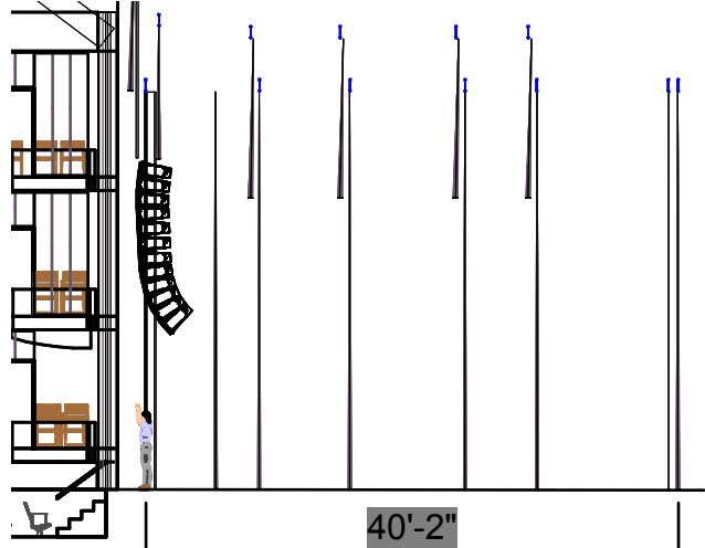
3 Lyric Stage Left View Scale: 1/16" = 1'-0"
